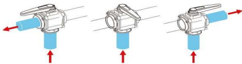
T-Port Configuration
