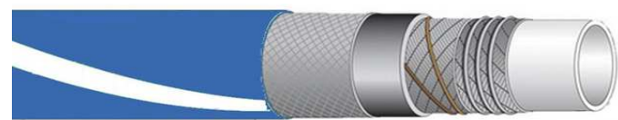
D710 - MAXFLO Acid & Chemical Suction/Delivery
