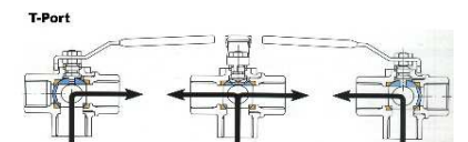
3110T - Brass T-Port 3-Way Ballvalve
