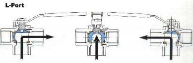
3210L - Brass L-Port 3-Way Ballvalve
